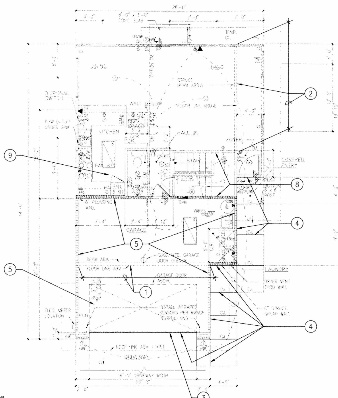
2 LOWER FLOOR PLAN S-1 SCALE: 1/4"=1'-0"
